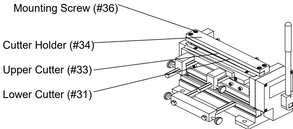
Figure 6 – Removing the upper Cutter
