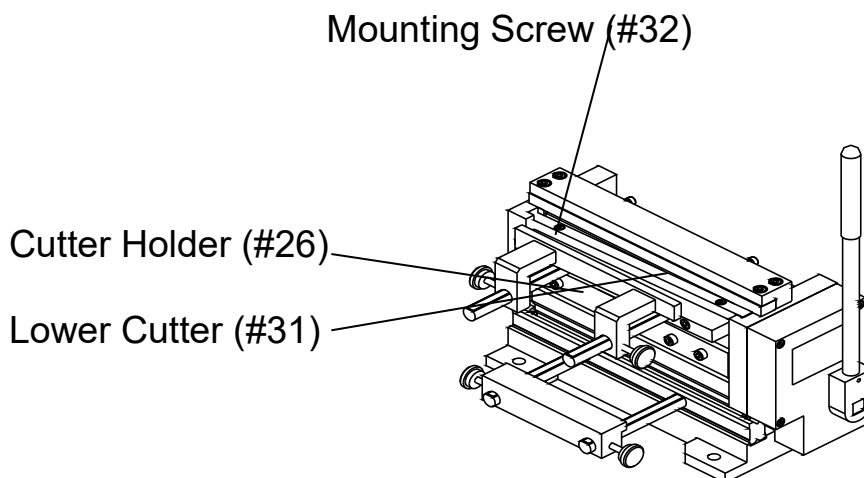
Figure 7 – Removing the Lower Cutter
