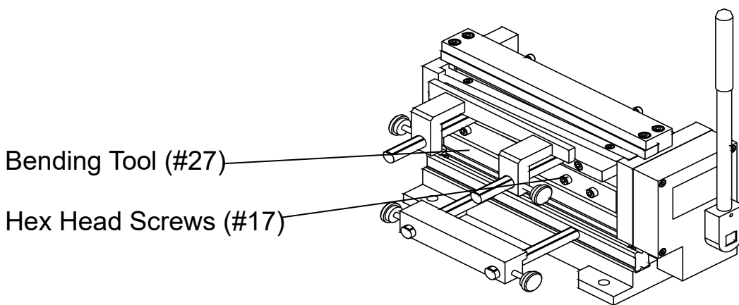
Figure 3 – Bending Tool Removal
