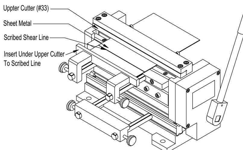
Figure 8 – Inserting scribed Sheet Metal
