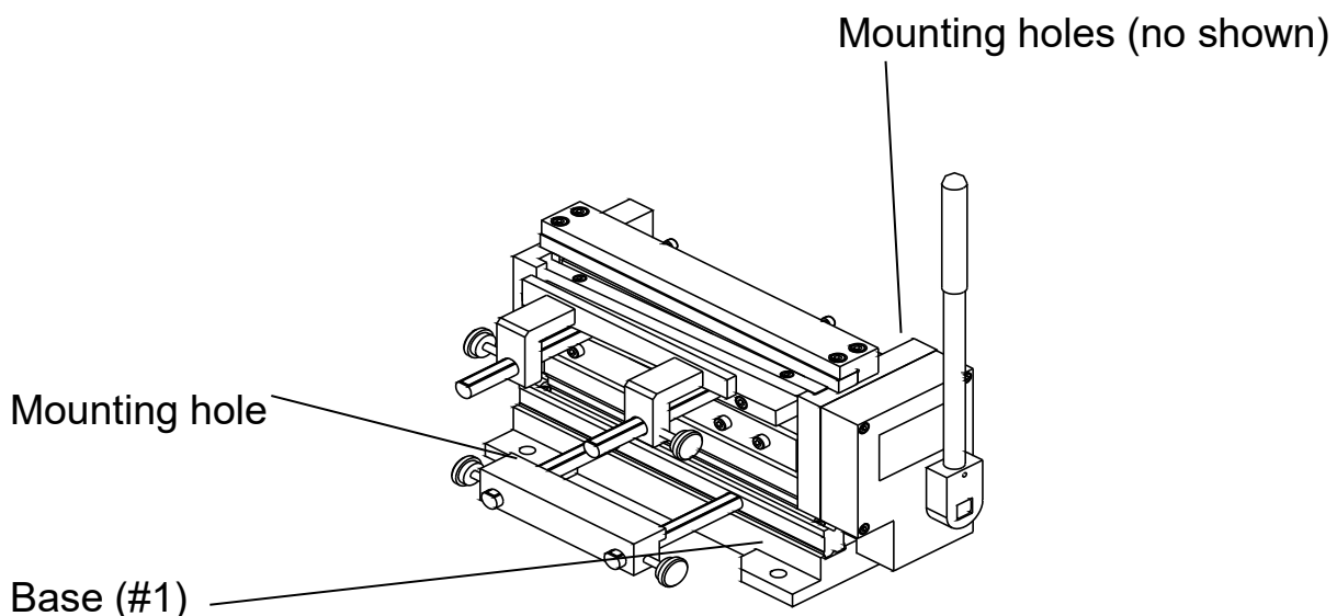
Figure 1 – Mounting Shear/brake to a Wood workbench
