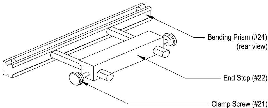
Figure 4 – Loosening the Clamp Screw
