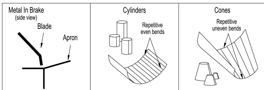
Figure 10 – Radius Bending
