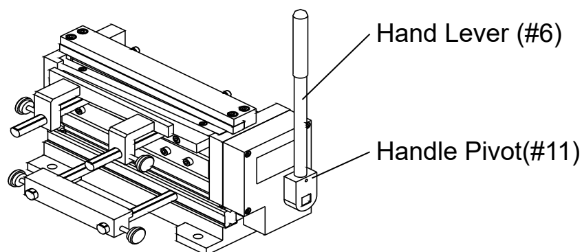
Figure 2 – Hand lever Installation
