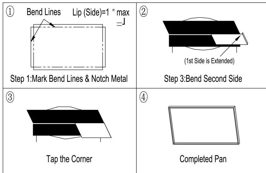
Figure 9 – Pan Forming
